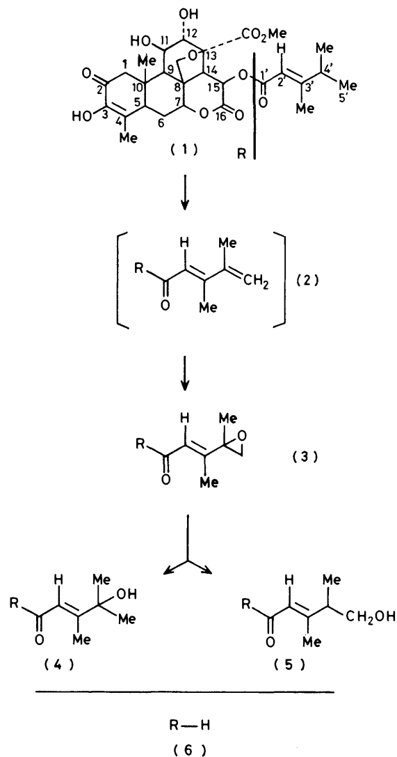
SCHEME Structures of bruceantin (1), microbial transformation products (3), (4), and (5), and bruceolide (6)
